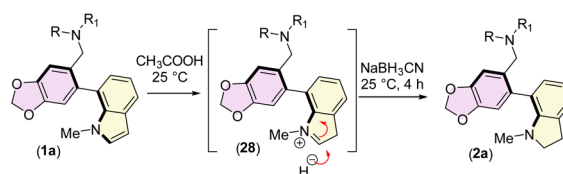
Scheme 7 Probable mechanism for the reduction of the indole ring.
