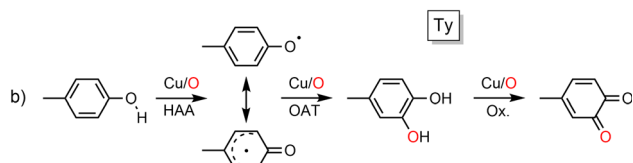
Scheme 1 Reaction type catalyzed by copper-containing mono-oxygenases (a) DβH (Dopamine β-monooxygenase); PHM (Peptidyl-glycine α-Hydroxylating Monooxygenase); pMMO (particulate Methane Monooxygenase); LPMO (Lytic Polysaccharide Monooxygenase); FGE (Formylglycine-Generating Enzyme) and (b) Ty (Tyrosinase).
