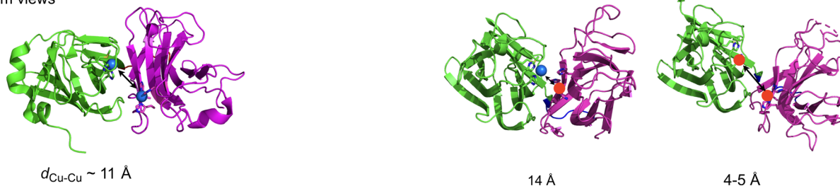
Fig. 2 Uncoupled binuclear copper-containing monooxygenases, PHM and DβH. (a) and (b) reactions catalyzed by PHM and DβH, respectively; (c) X-ray structure of PHM from Rattus norvegicus showing the two domains (Cu M domain in green and Cu H domain in magenta) connected by a loop (in blue) in which each domain binds a single copper atom spaced from each other by approximately 11 Å and (d) structure of the Cu M -superoxido intermediate in PHM (PDB ID 1opm); (e) and (f) X-ray structure of the human DβM (PDB ID 4zel) showing the open (e) and the closed (f) forms. Only the Cu M domain of the closed form contains a copper atom, the other copper ions (red sphere) are manually placed.
