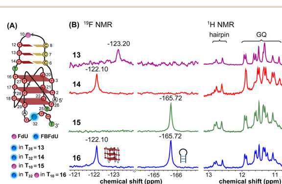
Fig. 4 (A) Schematic representation of the juxtaposed GQ-hairpin structure of the LTR-III + IV region. (B) 19 F NMR and partial 1 H NMR spectra of ONs 13–16.
