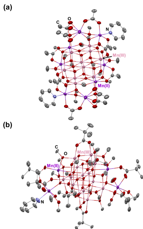
Fig. 1 Solid state structures of [Mn 18 -Ac] (a) and [Mn 18 -Piv] (b) drawn with thermal ellipsoids at the 30% probability level. Hydrogen atoms are omitted for clarity. Colour code: Mn II , purple; Mn III , pink; O, red; N, blue; C, grey.
