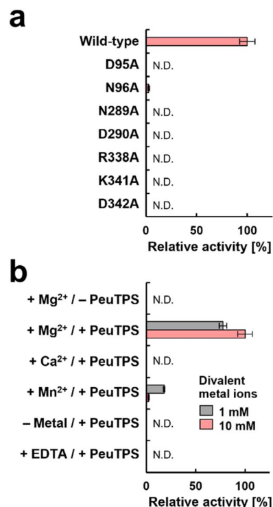
Fig. 5 Enzymatic activities of wild-type and variant PeuTPSs in converting the GGPP substrate to produce 1 and 2. Quantification of the products was performed using GC. Product ratios were not changed in all reactions. Error bars indicate standard deviation ( n = 3 ). N.D.: not detectable. (a) Comparison of enzymatic activities of variants with wild-type PeuTPS. (b) Analysis of requirements for divalent metal ions in the wild-type PeuTPS reaction. Concentrations of divalent metal ions were 1 or 10 mM. Reactions in the absence of divalent metal ions and in the presence of EDTA (10 mM) were also performed.
