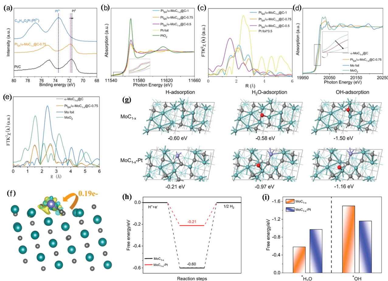
Fig. 6 (a) Pt 4f XPS spectra. (b) Pt L_{3-} -edge XANES spectra. (c) Fourier transform X-ray absorption fine structure (FT-EXAFS) curves. (d) Mo K-edge X-ray absorption near edge structure (XANES) spectra. (e) FT-EXAFS curves of the Mo K-edge. (f) Differential charge density for \text{Pt}_1/\alpha\text{-MoC}_{1-x} . (g) Optimized adsorption geometries. (h) Gibbs free energy diagram. (i) Calculated adsorption free energies. Reproduced with permission. 76 Copyright 2021, Wiley-VCH GmbH, Weinheim.
