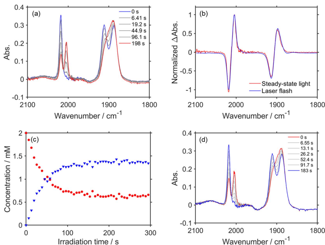
Fig. 4 (a) FT-IR spectra of \text{CO}_2 saturated DMSO-TEOA (5:1 v/v) solution containing RuC2Re (2.0 mM) and BIH (0.1 M) during steady-state light irradiation at 480 nm; d = 0.5 \text{ mm} . (b) Normalized TR-IR spectrum at 3.0 s after laser flash (blue) and FT-IR spectrum after steady-state light irradiation for 198 s (red). (c) Concentration changes of RuC2Re (red) and RuC2Re(COOH) (blue) during steady-state light irradiation. (d) FT-IR spectra of \text{CO}_2 saturated DMSO-TEOA (5:1 v/v) solution containing RuC2Re (2.0 mM) and BIH (0.1 M) after steady-state light irradiation ( \lambda = 480 \text{ nm} ) for 2 min.
