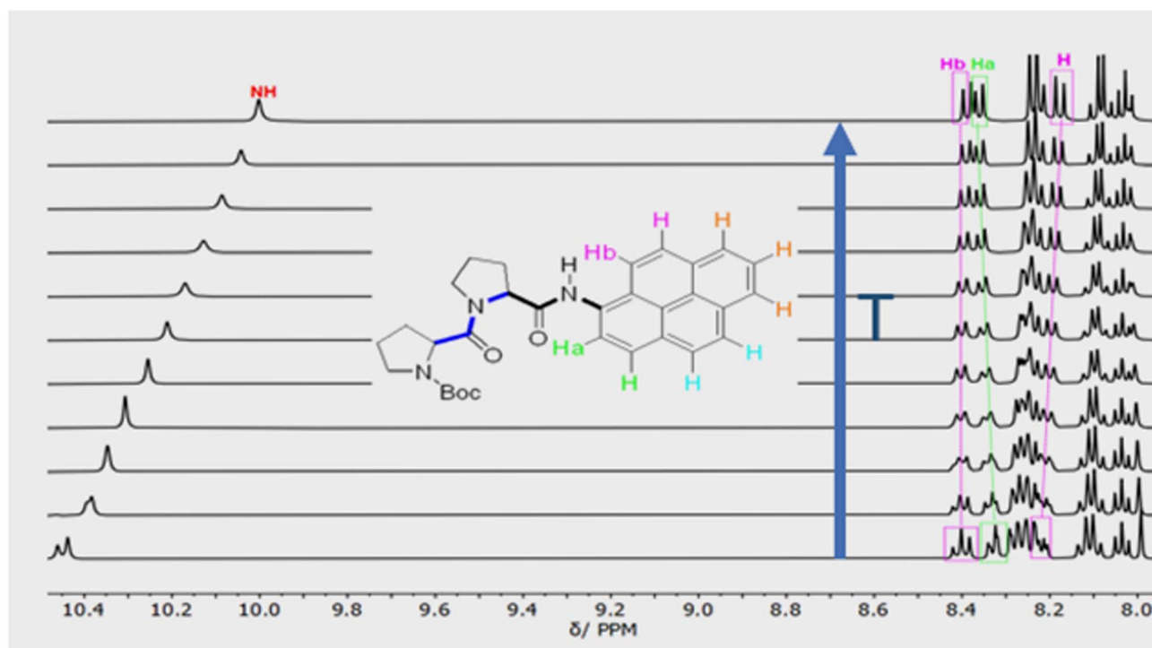
Fig. 3 Variable temperature ^1\text{H} NMR spectra of PY-P 2 in \text{D}_6 -DMSO showing the aromatic region and the most downfield proton resonances. The blue arrow indicates the direction of increasing temperature. The first spectrum was recorded at 298 K, the second at 313 K and subsequent spectra were recorded at intervals of 10 K until 403 K.
