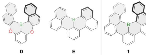
Fig. 1 Previously reported boron-doped helicenes and bora[6]helicene 1 presented herein.
