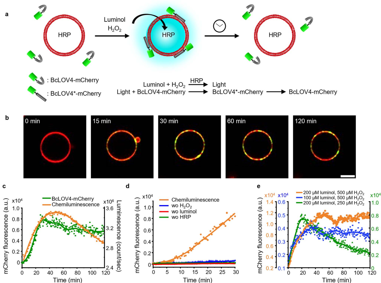
Fig. 5 (a) Schematic representation of BcLOV4-mCherry recruitment on a membrane with intravesicular chemiluminescence. (b) Confocal microscopy images of BcLOV4-mCherry (shown in green) recruitment kinetics on the membrane (DiD staining, shown in red). Scale bar is 10 \mu\text{m} . Also see Movie 2.† (c) Quantification of BcLOV4-mCherry on the membrane in (b) and chemiluminescence emission dynamics in GUVs as measured with a plate reader. (d) Negative controls for (b) where each of the reagents or catalyst for the chemiluminescence reaction was left out. (e) Comparison of BcLOV4-mCherry recruitment on the membrane with different substrate concentrations as in Fig. 4e.
