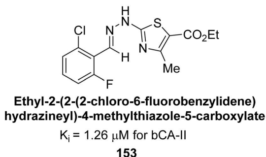
Fig. 51 Chemical structure of compound 153 and its K_i value against bCA-II along with its docking image.
