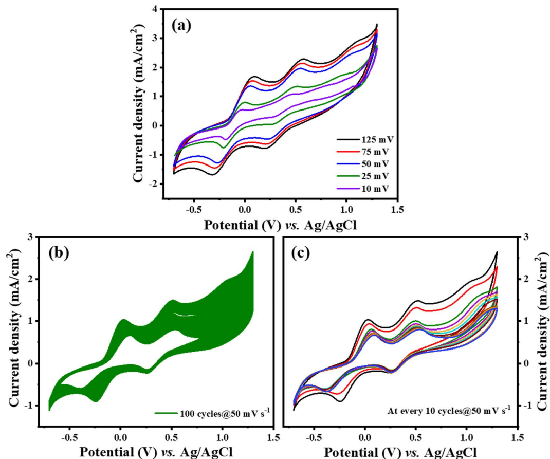
Fig. 6 (a) \text{Ti}_3\text{C}_2\text{T}_x\text{-PTh} at various scan rates (b) and (c) stability test of \text{Ti}_3\text{C}_2\text{T}_x\text{-PTh} at 50 \text{mV s}^{-1} for 100 cycles and plotted at every 10 cycles.
