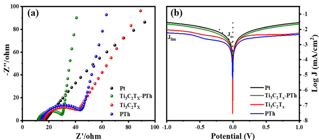
Fig. 7 (a) Electrochemical impedance spectra of Pt, \text{Ti}_3\text{C}_2\text{T}_x , PTh and \text{Ti}_3\text{C}_2\text{T}_x\text{-PTh} CE made from the symmetrical cell (b) Tafel polarisation of Pt, \text{Ti}_3\text{C}_2\text{T}_x , PTh and \text{Ti}_3\text{C}_2\text{T}_x\text{-PTh} CE.
