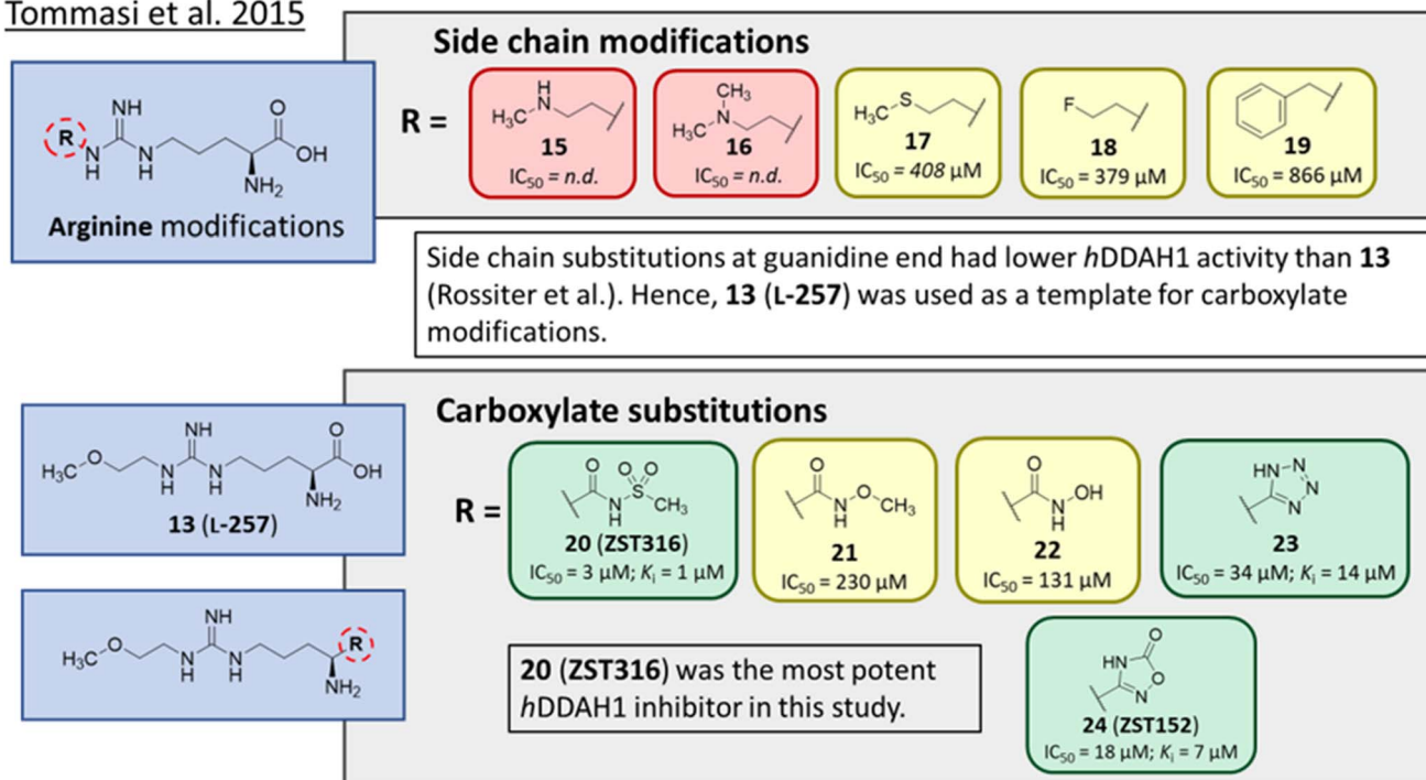
Fig. 3 Development of h DDAH1 inhibitor ZST316 ( 20 ) 22 from L-257 ( 13 ). 18 R group substitutions shown in green ( K_i and IC_{50} < 100 \mu M ); yellow ( IC_{50} = 100 – 1000 \mu M ) and red ( IC_{50} = n.d. ). n.d. = not determined when inhibition < 50\% at 1 mM.
