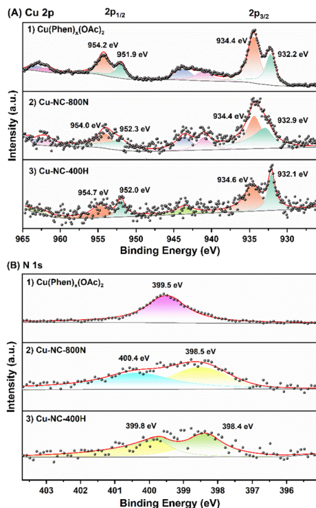
Fig. 5 The XPS of (A) Cu 2p signals: (1) Cu(Phen) x (OAc) 2 , (2) Cu-NC-800N, and (3) Cu-NC-400H samples and (B) N 1s signals: (1) Cu(Phen) x (OAc) 2 , (2) Cu-NC-800N, and (3) Cu-NC-400H samples.
