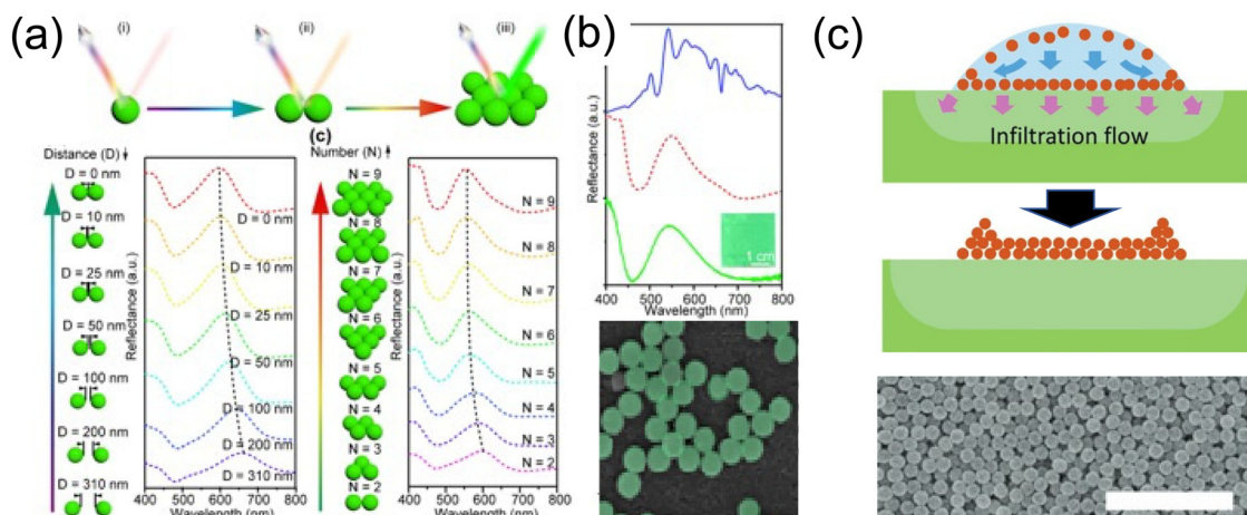
Fig. 18 (a) Schematic illustration of NIA and their reflection spectra with various configurations. (b) Simulated reflection spectrum of aggregates constructed of nine 310 nm dielectric spheres (red dotted line), experimental reflection (green solid line), and dark-field reflection (blue solid line) spectrum of aggregates constructed of 310 nm ZnS spheres (green solid line). The inset is the digital image of this aggregate and their false colored SEM image. [Reproduced from ref. 180, with permission from American Chemical Society, Copyright 2020]. (c) Schematic illustration of infiltration-driven nonequilibrium colloidal assembly and the resulted SEM. Scale bar: 2 μm. [Reproduced from ref. 181, with permission from Wiley-VCH Verlag GmbH & Co. KGaA, Weinheim, Copyright 2018].
