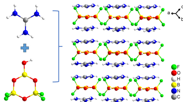
Fig. 15 Crystal structure of [C(NH_2)_3][B_3O_3F_2(OH)_2] .
