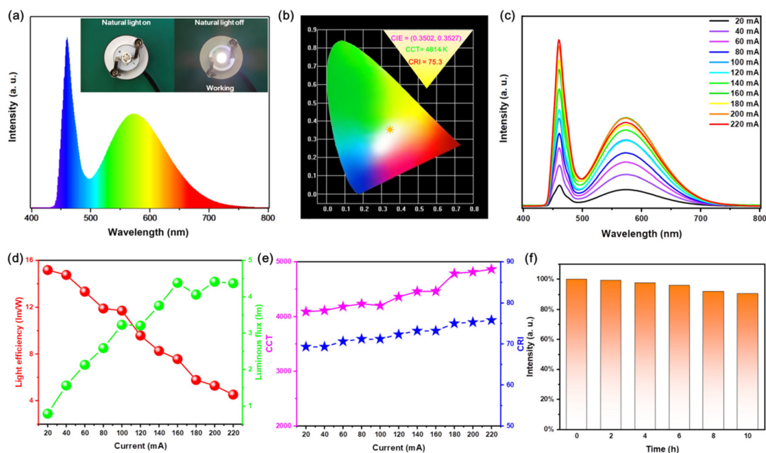
Fig. 10 (a) The PL spectrum of WLED device, and the inset for the working images of WLED; (b) the chromaticity parameter of WLED with 200 mA current; (c) PL spectra of WLED with different currents. (d) The optical efficiency and flux of WLED with different currents. (e) CCT and CRI of WLED with different currents. (f) Stability of WLED continuous operation.
