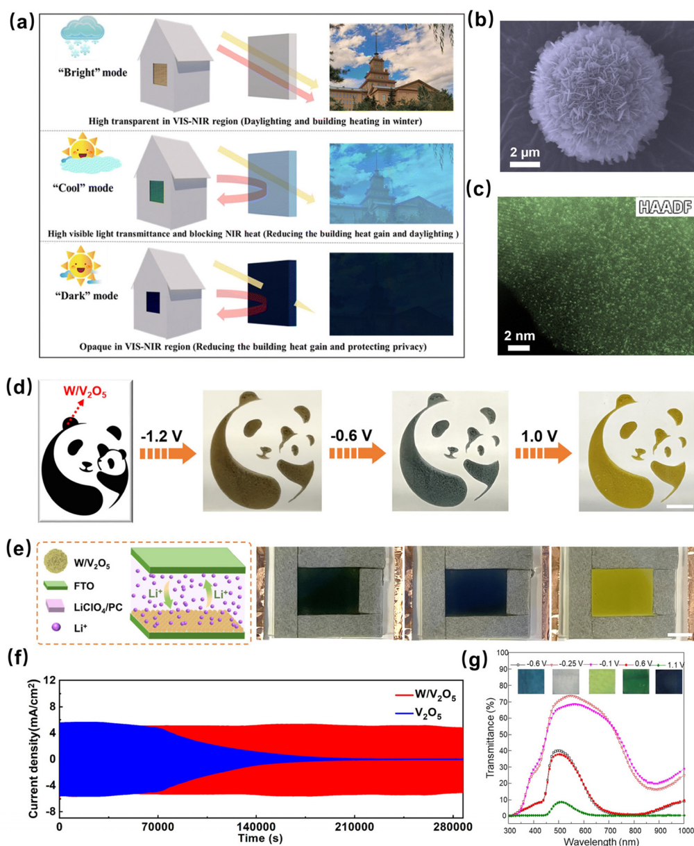
Fig. 9 (a) Application scenarios of the \alpha -WO 3-x O y electrochromic device in bright, cool, and dark operation modes. Reproduced with permission. 2 Copyright 2023, Royal Society of Chemistry. (b) SEM images of HLP-W/V 2 O 5 . (c) AC HAADF-STEM image of HLP-W/V 2 O 5 . (d) Prototype of the panda fabricated based on HLP-W/V 2 O 5 and photographs at different colored states. (e) Structural schematic diagram of the solid EC device and photographs of the solid EC device at different color states. (f) Cycling stability of HLP-W/V 2 O 5 and HLP-W/V 2 O 5 with multi-potential steps between -0.6 and 1 V for 79.4 h. Reproduced with permission. 17 Copyright 2023, Elsevier. (g) Transmittance of PANI-WO 3 thin films at different applied voltages. Reproduced with permission. 28 Copyright 2021, Elsevier.
