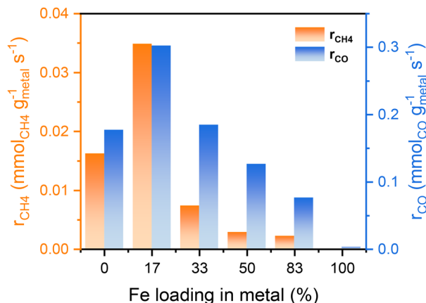
Fig. 3 Reaction rates of both methanation and RWGS after 16 h test for different Fe loadings in Ni 2 (Fe)/MgO catalysts.
