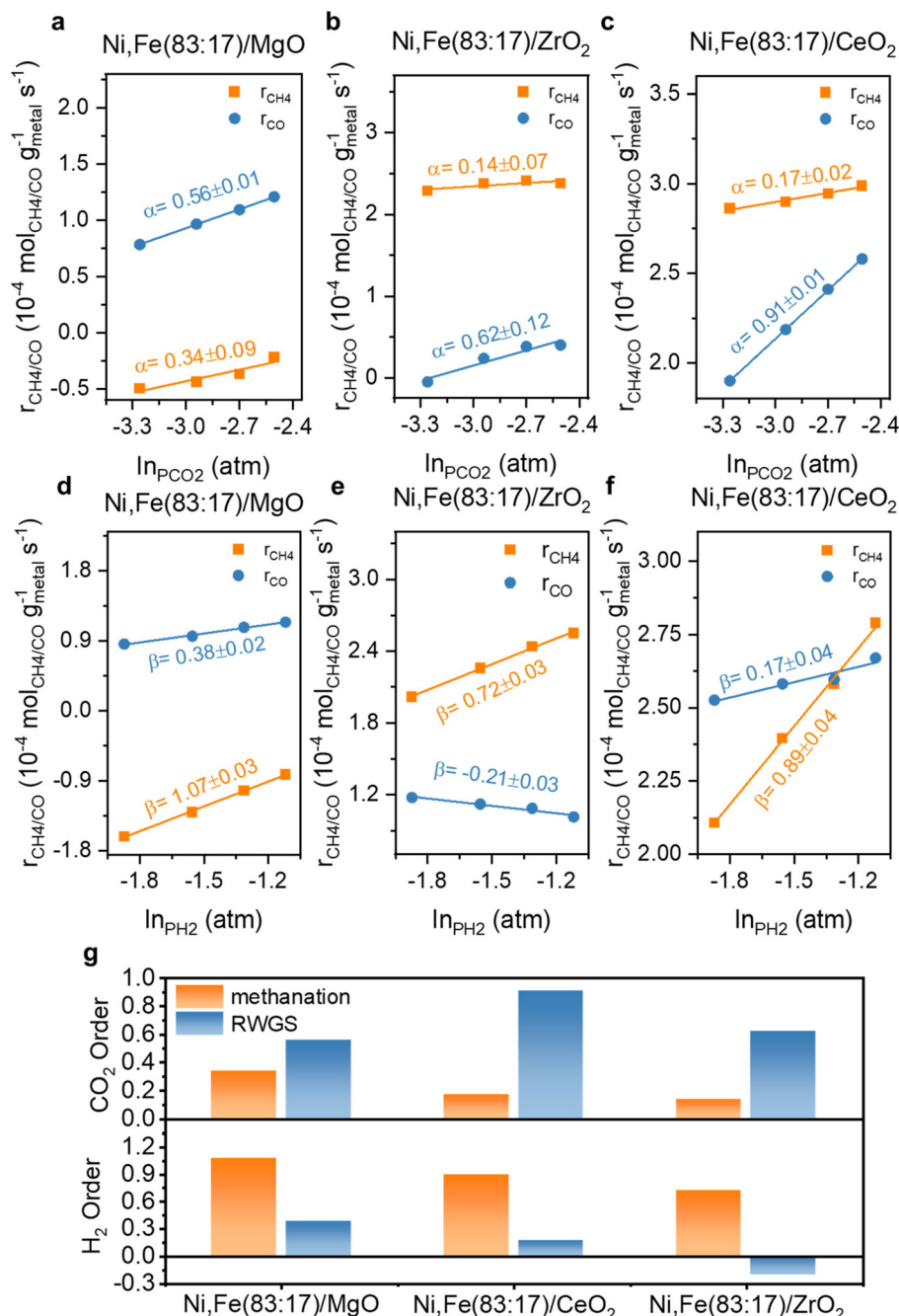
Fig. 11 The reaction order of \text{CO}_2 ( \alpha ) and \text{H}_2 ( \beta ) at 350 °C for Ni,Fe bimetallic catalysts supported on (a) & (d) MgO, (b) & (e) \text{ZrO}_2 and (c) & (f) \text{CeO}_2 and (g) their comparison.
