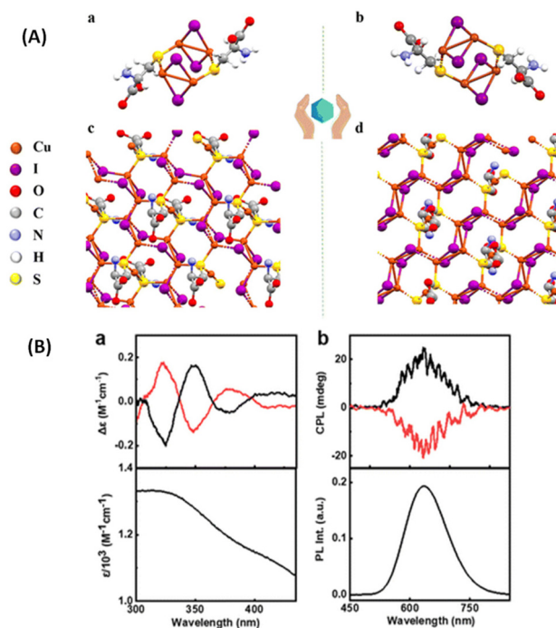
Fig. 12 (A) X-ray crystal structure of (a) (D\text{-Cys})_2\text{Cu}_4\text{I}_4 and (b) (L\text{-Cys})_2\text{Cu}_4\text{I}_4 nanoclusters and (B) experimental CD spectra (a) along with the corresponding absorption plot, and experimental CPL spectra (b) along with the corresponding luminescence spectra of the aqueous solution of nanoclusters. Black and red traces correspond to spectra collected from (D\text{-Cys})_2\text{Cu}_4\text{I}_4 and (L\text{-Cys})_2\text{Cu}_4\text{I}_4 nanoclusters, respectively. (Reproduced from ref. 51 with permission from the Royal Society of Chemistry, Copyright 2023).
