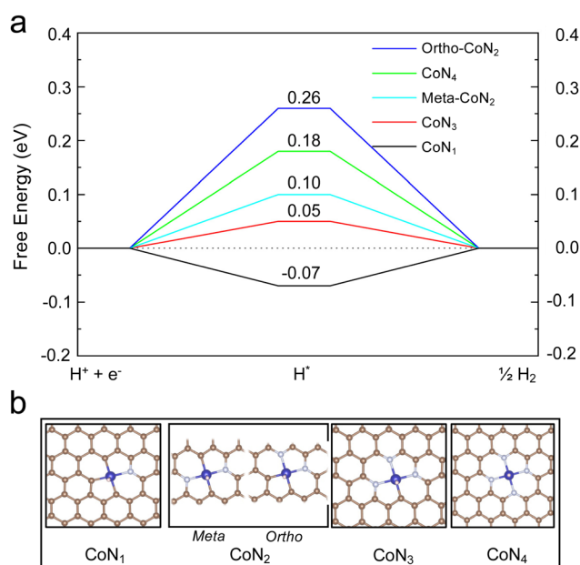
Fig. 5 DFT calculations of hydrogen adsorption. (a) Calculated HER free-energy diagram over different configurations of Co-N x -NAC. The H binding energy is labeled on top of each configuration. (b) Atomic structures of H adsorbed on Co-N x -NAC.
