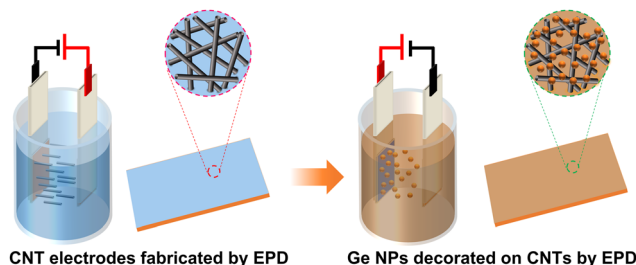
Fig. 1 Schematic illustration of the two-step process for the fabrication of Ge/CNT nanocomposite electrodes (fabrication of CNT electrodes and decoration of Ge NPs on CNT electrodes) by using EPD.
