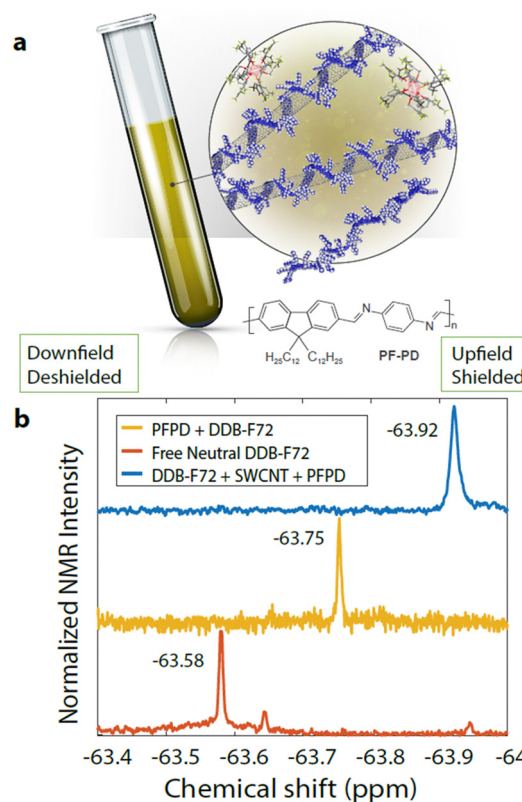
Fig. 2 (a) Cartoon showing the NMR tube sample composition: polymer dispersed s-SWCNT, excess polymer (in blue) and DDB-F72 molecules associated with a hole on the doped s-SWCNTs. Repeating unit of the polymer PF-PD is also presented for clarity. (b) Spectra corresponding to 19 F NMR for neutral DDB-F72 dopant in d 8 -toluene (6 \mu M, bottom), PF-PD polymer used to disperse s-SWCNTs with added DDB-F72 (6 \mu M, middle), and dispersed s-SWCNTs with added DDB-F72 (6 \mu M, top). Numbers show specific chemical shift.
