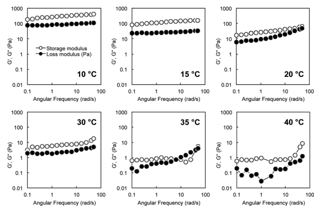
Fig. 2 Angular frequency dependence ( \text{rad s}^{-1} ) of storage modulus G' (open circles) and loss modulus G'' (closed circles) of G\text{-Py}^+ / S\text{-PEG}_{200}\text{-S} (10 mM/6 wt%) hybrid hydrogels at various temperatures and 0.25% strain.
