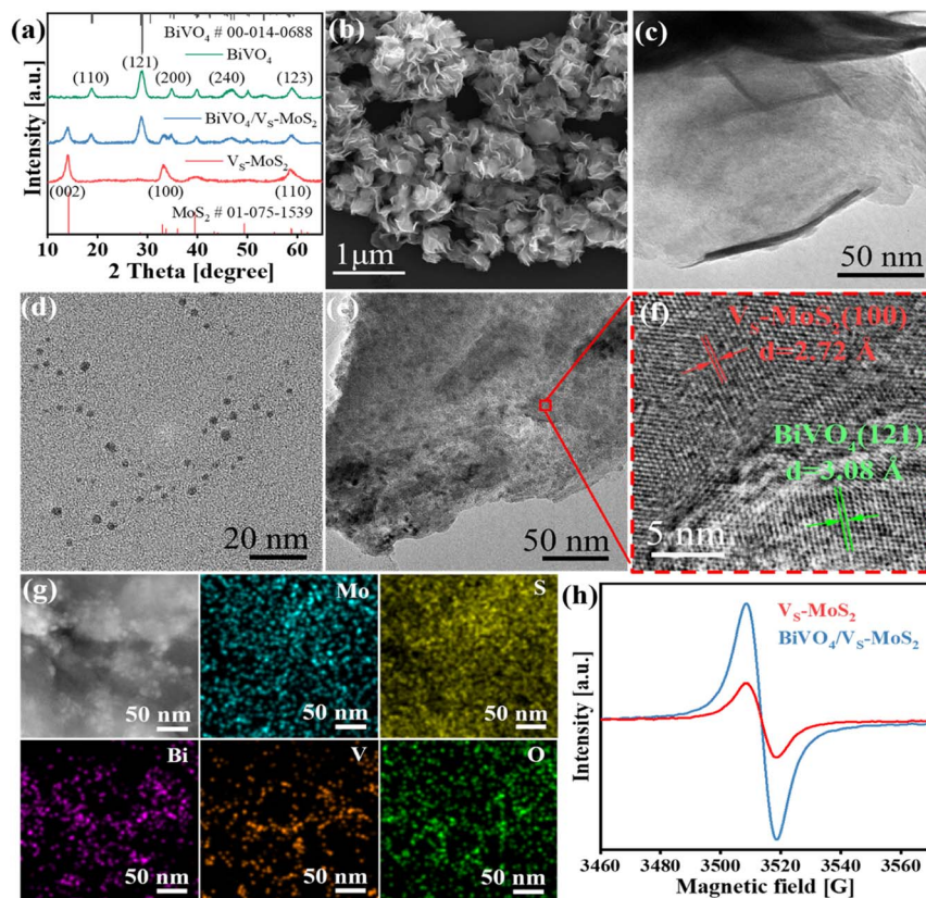
Fig. 1 (a) XRD patterns of V_S -MoS 2 , BiVO 4 , and BiVO 4 /V S -MoS 2 . (b and c) SEM and TEM images of a V_S -MoS 2 nanosheet. (d) TEM image of a BiVO 4 nanocrystal. (e–g) TEM, HRTEM, and corresponding EDS images of BiVO 4 /V S -MoS 2 . (h) EPR spectra of V_S -MoS 2 and BiVO 4 /V S -MoS 2 .
