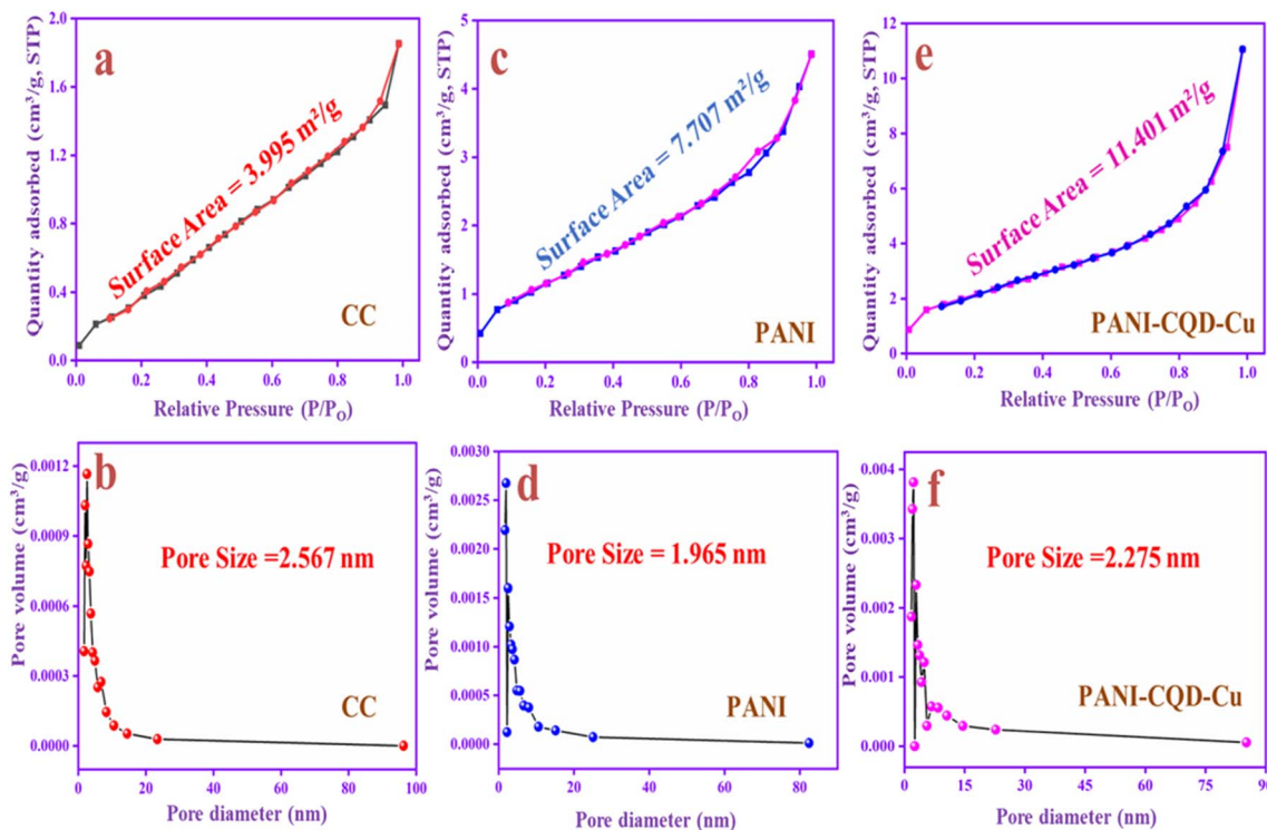
Fig. 8 N_2 adsorption isotherms and pore size distributions of CC (a and b), PANI (c and d) and PANI-CQD-Cu (e and f).
