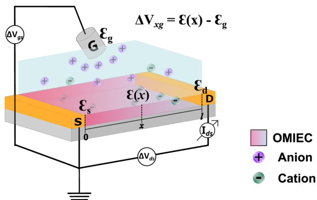
Fig. 1 Schematic representation of a typical OEECT structure.
