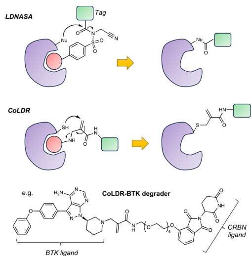
Fig. 3 Heterobifunctional ligand-directed protein surface labelling strategies using cleavable electrophilic warheads: ligand-directed N -acyl- N -alkylsulfonamide (LDNASA) and covalent ligand directed release (CoLDR). A BTK-directed CoLDR degrader probe based on the BTK inhibitor ibrutinib is shown.
