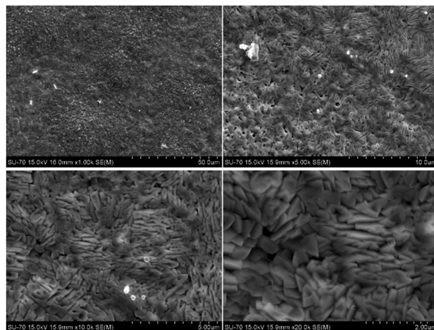
Fig. 9 SEM images of the sweep side of the CGO20C membrane captured after a \text{CO}_2 -separation test at different magnifications.
