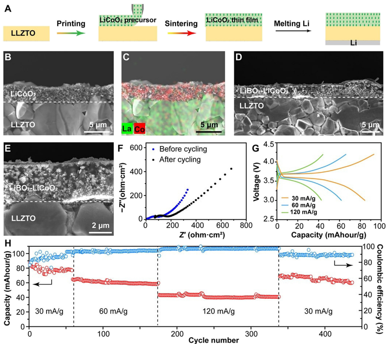
Fig. 10 (A) The printing and sintering process of the PRH-fabricated solid-state battery. (B) Cross-sectional SEM image and (C) EDS mapping of the PRH-sintered LCO cathode on the LLZO surface. (D) Cross-sectional and (E) magnified SEM images of the \text{LiBO}_2\text{-LCO/LLZO} interface. (F) EIS spectra of the all-solid-state battery ( \text{LiBO}_2\text{-LCO/LLZO/Li} ) before cycling and after the 450th cycle. (G) Voltage profiles of the in situ fabricated all-solid-state battery at different current densities. (H) Cycling performance and coulombic efficiency of the \text{LiBO}_2\text{-LCO/LLZO/Li} all-solid-state battery at 60 °C. 159 Copyright reprinted with permission from AAAS.
