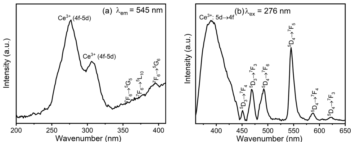
Fig. 5 (a) Excitation spectrum monitored at an emission wavelength of 545 nm and (b) emission spectrum excited at 276 nm of the CMC functionalized \text{Fe}_3\text{O}_4@SiO_2@GdPO_4:Tb^{3+}, Ce^{3+} nanocomposite.
