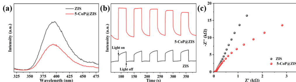
Fig. 6 (a) Steady-state PL spectra. (b) Transient photocurrent response curves. (c) EIS plots of ZIS and 5-CoP@ZIS.
