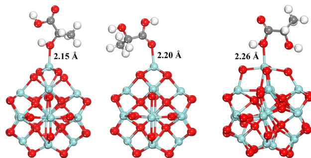
Fig. 11 Optimised structures of lactic acid adsorbed on the \text{ZrO}_2 nanocluster via (a) the oxygen atom of the alcohol functional group and (b and c) the carboxyl group. Here, white, red, grey, and cyan colour balls represent hydrogen, oxygen, carbon, and zirconium atoms, respectively.
