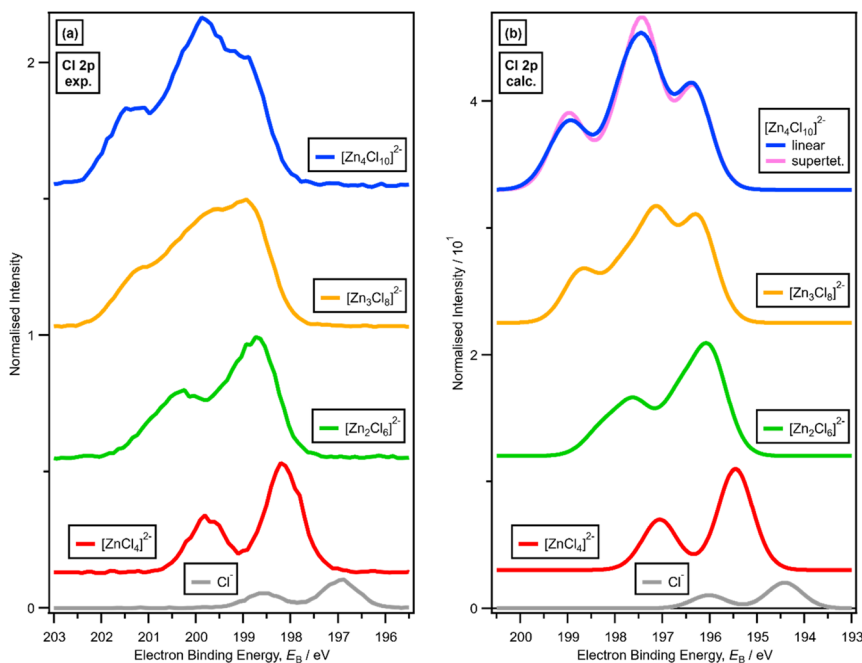
Fig. 6 (a) Experimental core Cl 2p XPS (going from bottom to top) for x = 0.00 [C 8 C 1 Im] 2 Cl, x = 0.33 [C 8 C 1 Im] 2 [ZnCl 4 ], x = 0.50 [C 8 C 1 Im] 2 [Zn 2 Cl 6 ], x = 0.60 [C 8 C 1 Im] 2 [Zn 3 Cl 8 ] and x = 0.67 [C 8 C 1 Im] 2 [Zn 4 Cl 10 ] (vertically offset for clarity). (b) Lone ion SMD calculated core Cl 2p XPS (going from bottom to top) for Cl - , [ZnCl 4 ] 2- , [Zn 2 Cl 6 ] 2- , [Zn 3 Cl 8 ] 2- and [Zn 4 Cl 10 ] 2- (vertically offset for clarity).
