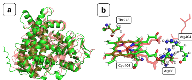
Fig. 2 (a) Backbone alignment of AlphaFold entry A0A2N0DV48 (green) and PDB entry 7WZL (red); (b) heme environment with important neighbouring residues for the aligned structures; 7WZL is in red, and AlphaFold entry A0A2N0DV48 uses the indicated atomic colours. Colours: green, carbon; red, oxygen; blue, nitrogen; yellow, sulphur; orange, iron; white, hydrogen.
