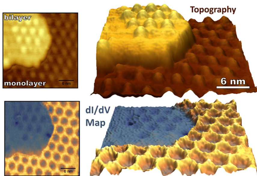
Fig. 5 Topography (top) and conductance mapping (bottom) of pristine monolayer and bilayer graphene on Ru(0001) is shown ( -1.5\text{ V} , -250\text{ pA} ). The bias was modulated with an amplitude of 200\text{ mV} to generate the dI/dV map. Note that atop regions of the single-layer graphene moiré pattern and the entirety of the bilayer graphene show lower conductance than the HCP and FCC regions of the G/Ru(0001) moiré pattern.
