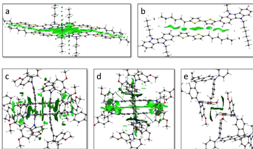
Fig. 5 Non-covalent interactions (NCI) surface plots of the reduced density gradient calculated using promolecular densities for relevant dimers of IDIDF in directions 100 (a) and 2\bar{1}\bar{1} (b), and spiro-OMeTAD in directions 100 (c), 000 (d) and 010 (e). The electronic couplings calculated for dimers a–e were 63, 17, 32, 7 and 5 meV, respectively.
