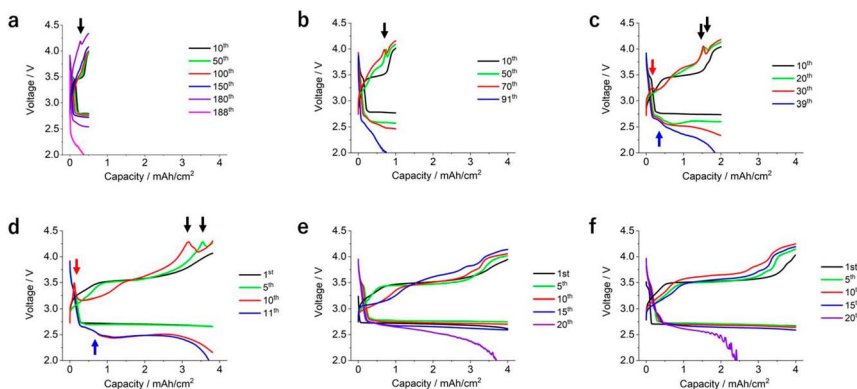
Fig. 1 Discharge/charge profile of LOB cells with different capacity limitation and current density conditions. (a) 0.05 \text{mA cm}^{-2} , 0.5 \text{mA h cm}^{-2} , (b) 0.1 \text{mA cm}^{-2} , 1 \text{mA h cm}^{-2} , (c) 0.2 \text{mA cm}^{-2} , 2 \text{mA h cm}^{-2} , (d and f) 0.4 \text{mA h cm}^{-2} , 4 \text{mA h cm}^{-2} and (e) 0.1 \text{mA cm}^{-2} , 4 \text{mA h cm}^{-2} . (f) 0.4 \text{mA h cm}^{-2} , 4 \text{mA h cm}^{-2} and a ceramic-based solid-state separator sandwiched between two pieces of a PO-based separator were adopted as the protective layer for the lithium metal electrode.
