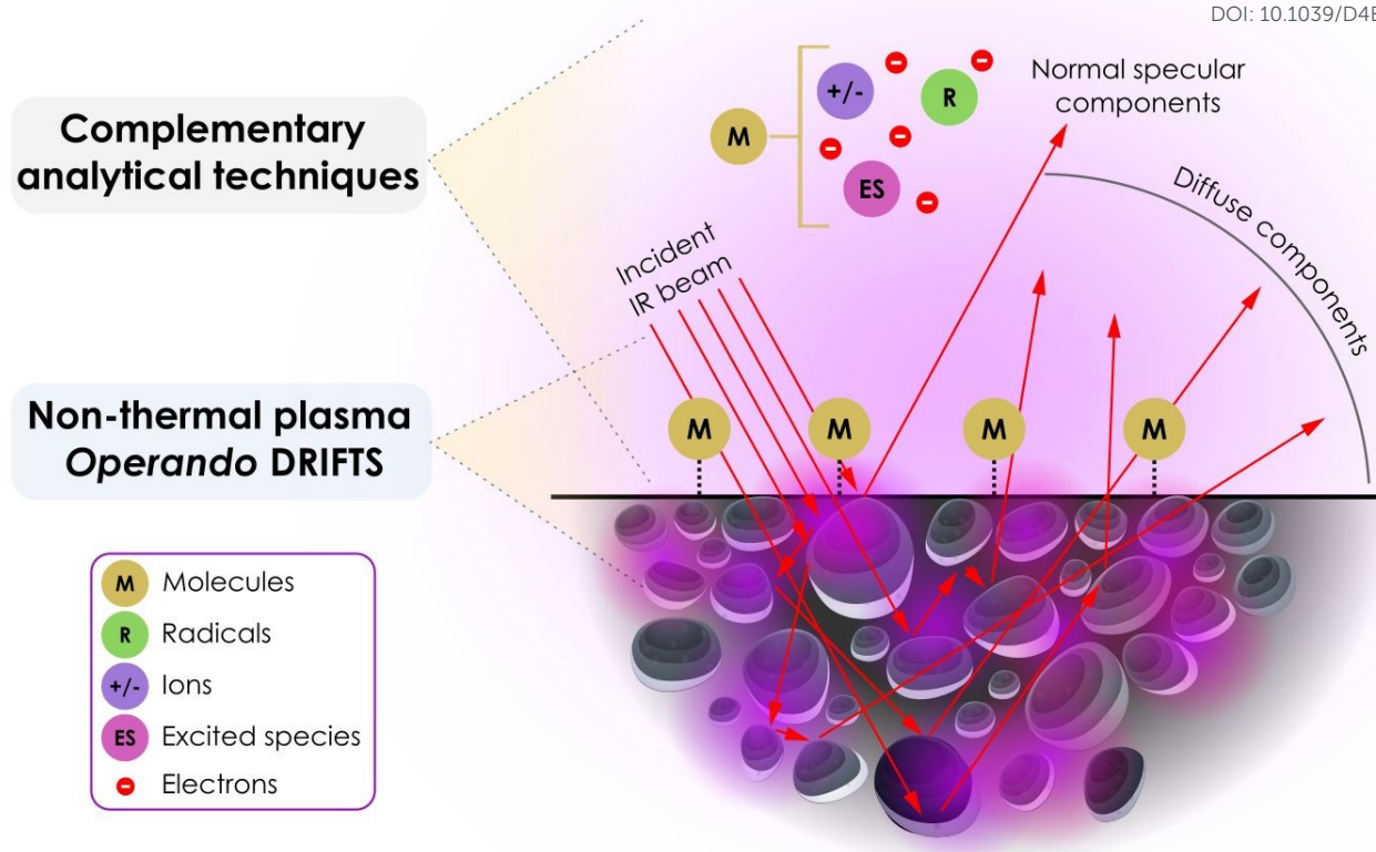
Figure 1. Processes responsible for producing the diffuse reflected infrared spectrum of adsorbates on a powder catalyst. Purple regions represent schematically the presence of local plasma discharge zones, while red arrows represent infrared beam lines. Modified from Armaroli et al. 19
