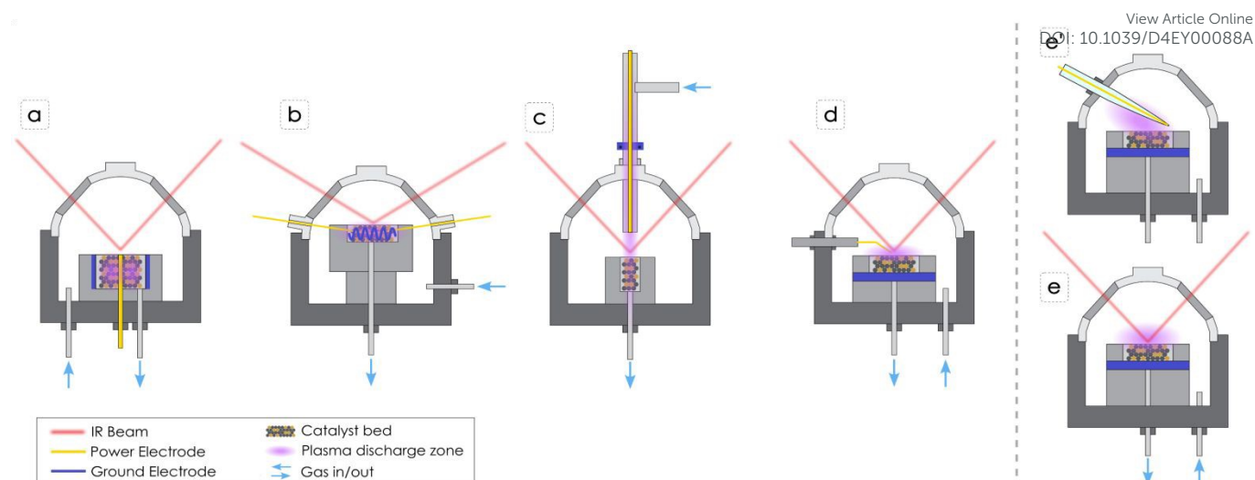
Figure 2: Schematic of operando DRIFTS configurations developed by research groups for investigating plasma catalysis at reaction conditions. (a) DBD embedded within the catalyst bed, (b) helical surface DBD, (c) DBD above the catalyst bed, (d) point-source DBD, (e, e') point-source DBD with two different views (this study). The dielectric is: a) the quartz capillary covering the power electrode, b) a coating on the power electrode, c) the quartz tube containing the plasma discharge zone, d) the sample holder depicted in light grey, e, e') the quartz tube covering the power electrode tip.
