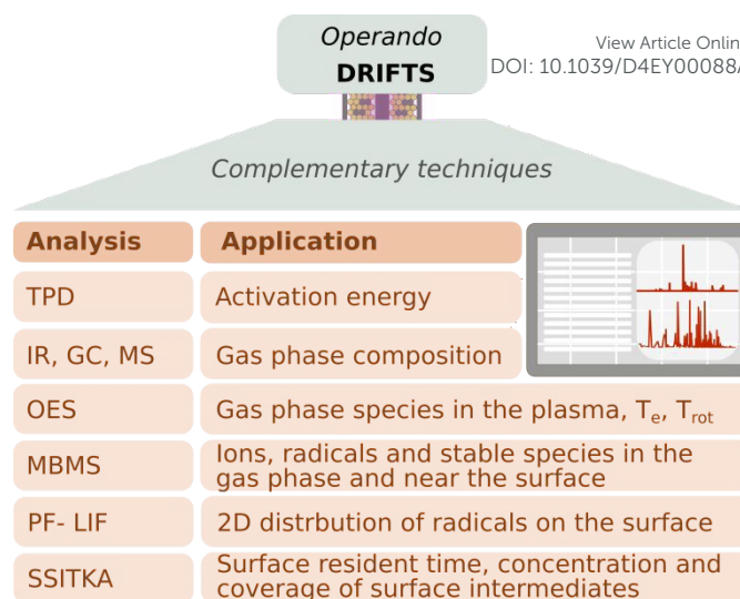
Figure 3: Scheme highlighting analytical techniques complementary to operando DRIFTS: Temperature-Programmed Desorption (TPD), Infrared (IR) or Mass Spectrometry (MS), Optical Emission Spectroscopy (OES), Molecular Beam Mass Spectrometry (MBMS), Photofragmentation Laser-Induced Fluorescence (PF-LIF), Steady-State Isotopic Transient Kinetic Analysis (SSITKA).
