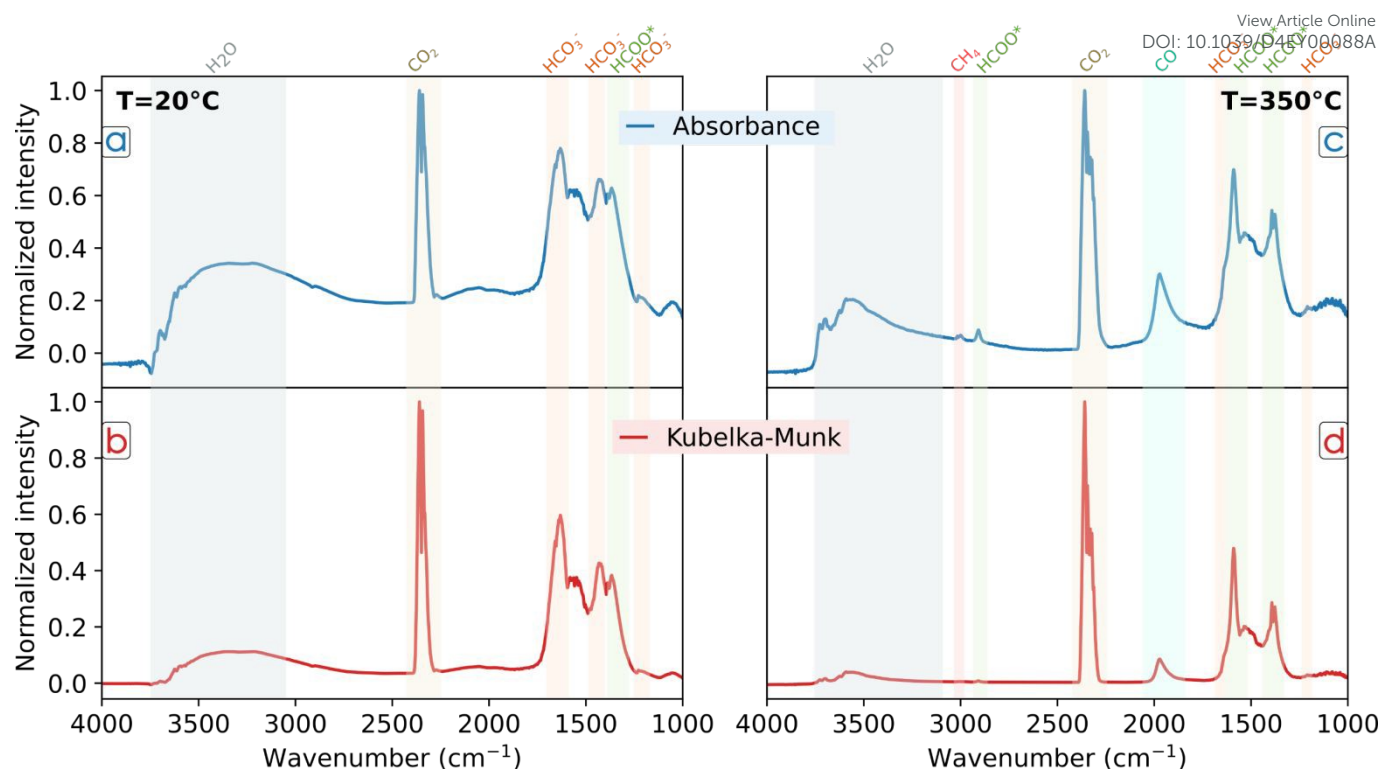
Figure 4. Comparison of Absorbance vs Kubelka-Munk spectra taken during NTP CO 2 hydrogenation over Co/Al 2 O 3 . DRIFTS cell temperature was controlled at 20°C (a, b) and 350°C (c, d). Data were collected in a custom modified plasma DRIFTS cell with NTP at 4000 V and 10 kHz with 36 sccm of Ar, 1 sccm of CO 2 and 3 sccm of H 2 .
