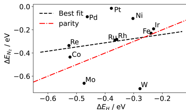
Fig. 8 Scaling of dinitrogen binding with hydrogen binding energetics.
