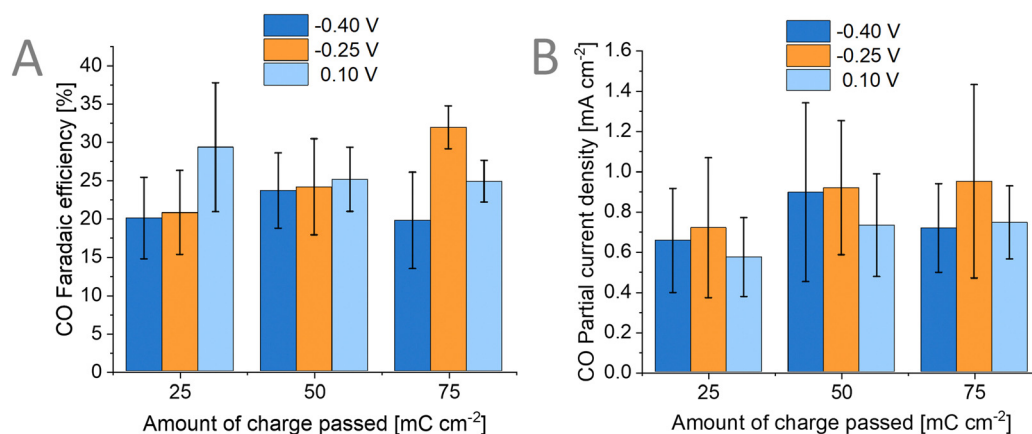
Fig. 7 (A) Faradaic efficiency for CO of the FTO/Au/Sb 2 Se 3 /TiO 2 /Au photoelectrode with corresponding (B) partial current density for CO at different deposition bias ( -0.4 \text{ V} , -0.25 \text{ V} , 0.1 \text{ V vs. Ag/AgCl} ) and different amount of charge passed (25, 50, 75 \text{ mC cm}^{-2} ) for the Au catalyst deposition.
