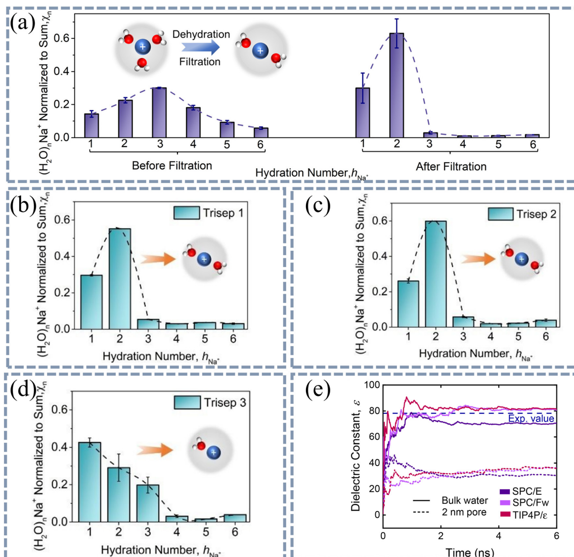
Fig. 4 Steric effects or dielectric effects lead to dehydration of ions. (a) Variation of hydration number ( h_{\text{Na}^+} ) of \text{Na}^+ ions before and after filtration of 10 mM NaCl solutions by NF90 (effective channel radius: 0.22 nm). h_{\text{Na}^+} of \text{Na}^+ ions after filtration of 10 mM NaCl solution by (b) Trisep 1 (effective channel radius: 0.29 nm), (c) Trisep 2 (effective channel radius: 0.30 nm), and (d) Trisep 3 (effective channel radius: 0.58 nm). Dehydration occurs when \text{Na}^+ ions pass through all four membranes. Reproduced from ref. 69 with permission from American Chemical Society, copyright 2021. (e) MD simulations of the dielectric constant of bulk and nanoconfined water by the rigid three-site SPC/E, flexible three-site SPC/Fw, and rigid four-site TIP4P/ \epsilon water models. For bulk water, the dielectric constant is \sim 80 . For water molecules in 2 nm pores, the dielectric constant is \sim 30 .
