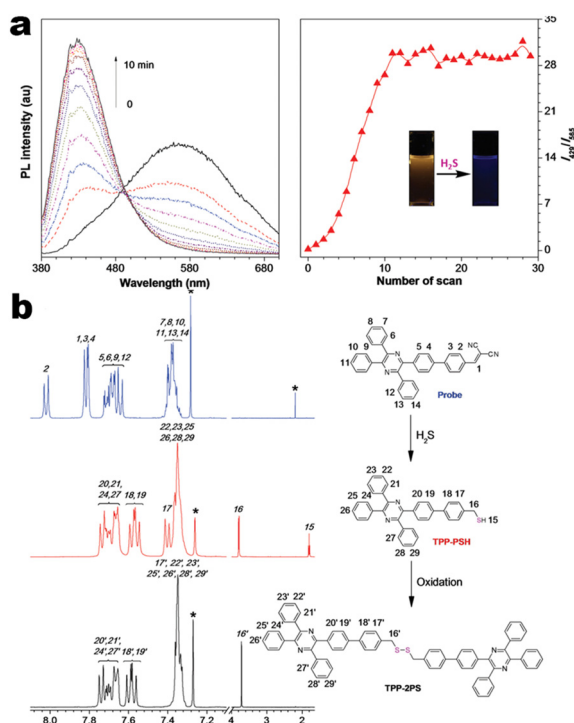
Fig. 8 (a) Time-dependent PL spectra of 2-14 treated with NaHS in DMSO/PBS buffer mixture. (b) ^1\text{H} -NMR spectra of 2-14 and possible reaction intermediate. Reproduced from ref. 77 with permission. Copyright (2018), Wiley Online Library.
