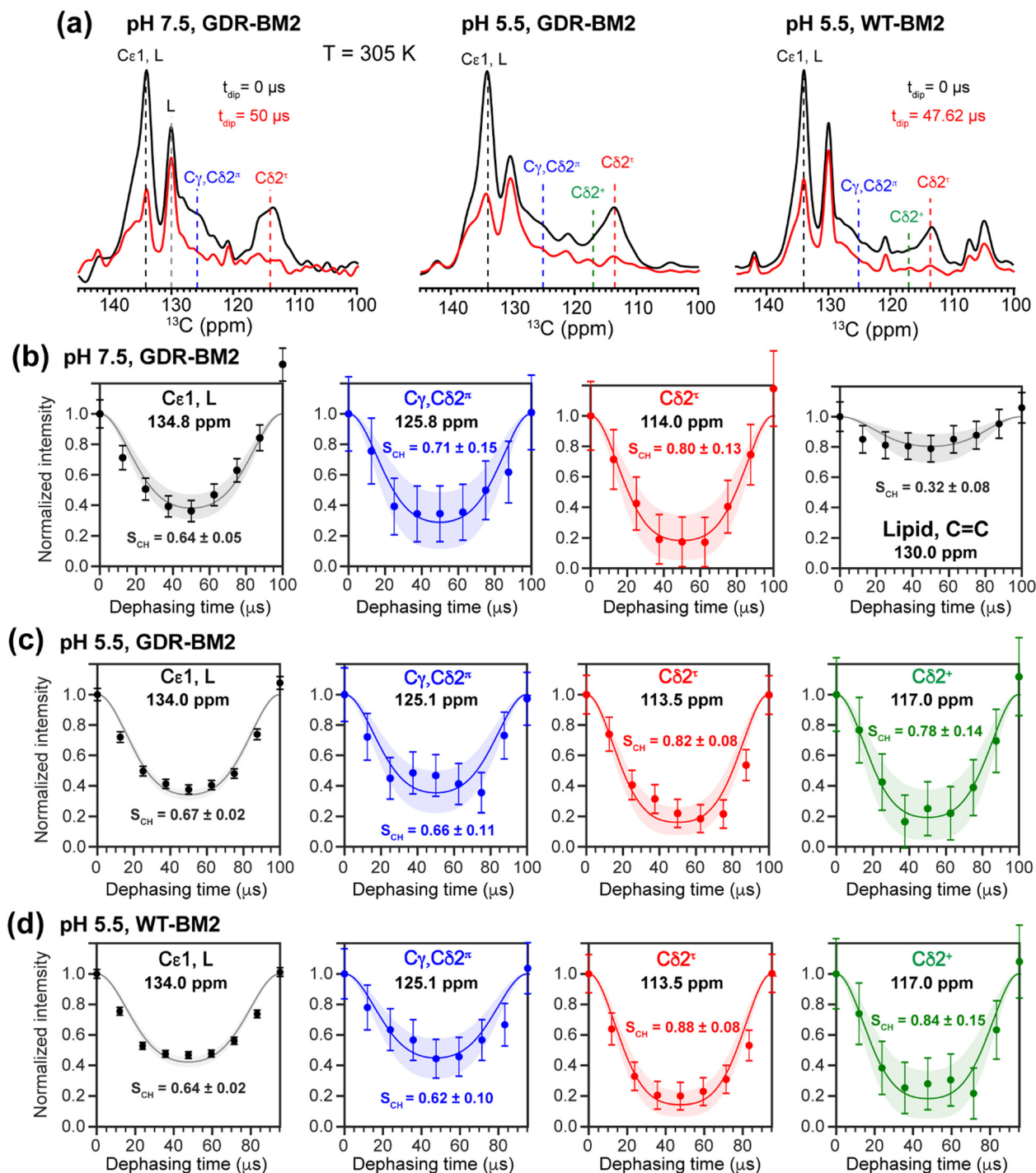
Fig. 6 2\text{D }^{13}\text{C}-^1\text{H} DIPSIFT data of membrane-bound GDR-BM2 and WT-BM2. The spectra were measured at 305 K under 10 kHz or 10.5 kHz MAS. (a) Aromatic region of the ^{13}\text{C} dimension of the 2D spectra of the three peptides at C-H dipolar evolution times of 0 \mu\text{s} and half of the rotor period (50 \mu\text{s} or 47.6 \mu\text{s} ). (b) C-H dipolar dephasing of GDR-BM2 at pH 7.5. (c) C-H dipolar dephasing of GDR-BM2 at pH 5.5. (d) C-H dipolar dephasing of WT-BM2 at pH 5.5. Error bars were propagated from the spectral signal-to-noise ratios. Best-fit simulations (solid lines) are shown along with uncertainties in the S_{\text{CH}} values (shaded areas) up to two standard deviations. The rigid-limit C-H dipolar coupling is assumed to be 23.9 kHz.
