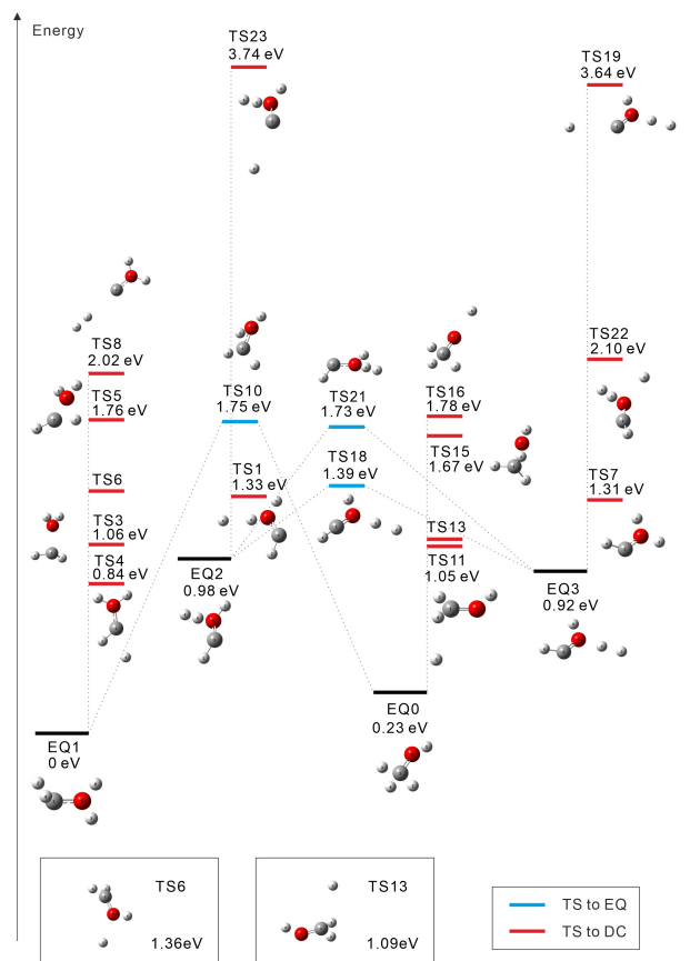
Fig. 2 Calculated isomerization and dissociation pathways for the triplet dication \text{CH}_3\text{OH}^{2+} (red: O, gray: C, and white: H). \text{EQ}_i , \text{TS}_i : equilibrium geometry and transition state, respectively. The energy difference from the neutral ground state to the dication \text{EQ}_0 is calculated to be +30.34 eV for the triplet state (including the ZPVE correction). Due to space limitations, two TSs are shown in boxes.
