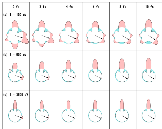
Fig. 5 Snapshots of PA-MFPADs averaged over 200 trajectories for the \text{H}^+ ejection at photoelectron energies (a) 100 eV, (b) 500 eV, and (c) 2.5 keV. The arrows indicate the angles averaged over 200 trajectories for the position of \text{H}^+ ejected in each time frame. We set the O atom at the origin, the C atom on the z axis ( z > 0 ), and the ejected \text{H}^+ on the zx plane, i.e., the plane of the figure ( x > 0 ).
