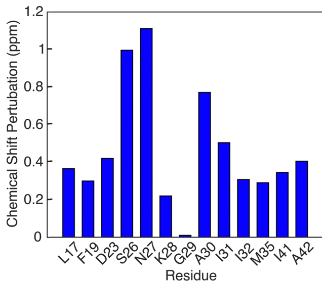
Fig. 6 Chemical shift perturbations of E22G \text{A}\beta_{1-42} fibrils relative to wild type \text{A}\beta_{1-42} fibrils found in [ref. 23, 38, 50].
