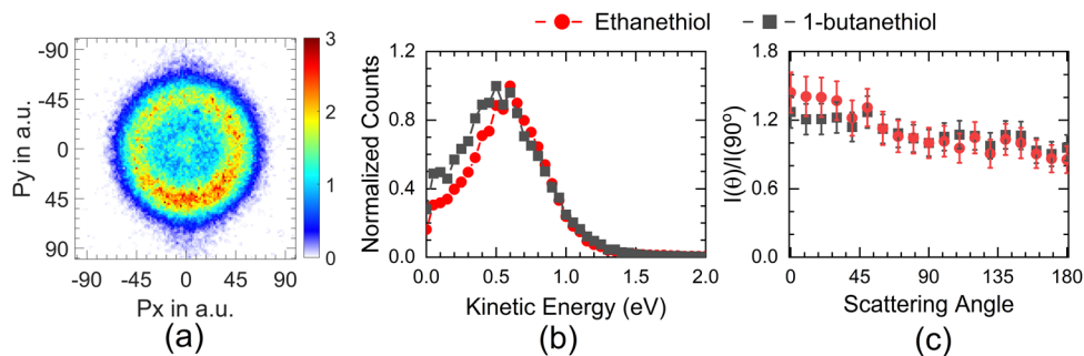
Fig. 7 (a) Momentum image obtained for the S^- + SH^- channel from 1-butanolthiol at 8 eV. Corresponding (b) KE and (c) angular distribution of the S^- + SH^- channel from 1-butanolthiol (—■—) along with those for ethanethiol (—●—).
