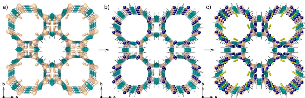
Fig. 2 Design approach showing the crystal structures of (a) 1, (b) 2, and (c) 3, showing the two-step post-synthetic process of the formation of Ag 2 @MOF. Cu and Ni atoms from the network are represented by cyan and orange polyhedra, respectively, whereas organic ligands are depicted as gray sticks. Orange, yellow, and blue spheres represent Ni, Na, and Ag atoms, respectively. Reprinted with permission from Tiburcio et al. Copyright 2022 American Chemical Society.
