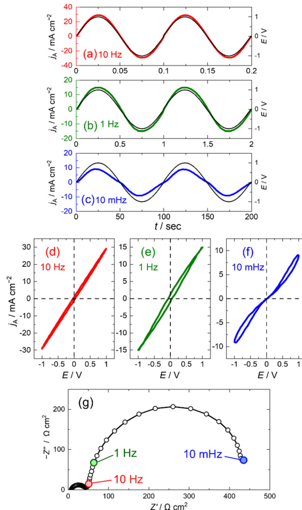
Fig. 2 (a)–(c) Applied voltage and output current for polarisation measurements; (d)–(f) steady-state polarisation curves of a LAMO/LAMO symmetric cell at -15\text{ }^{\circ}\text{C} . The frequency of applied voltage was (a) and (d) 10 Hz, (b) and (e) 1 Hz and (c) and (f) 10 mHz. (g) The Nyquist plot of the LAMO/LAMO symmetric cell measured at -15\text{ }^{\circ}\text{C} .
