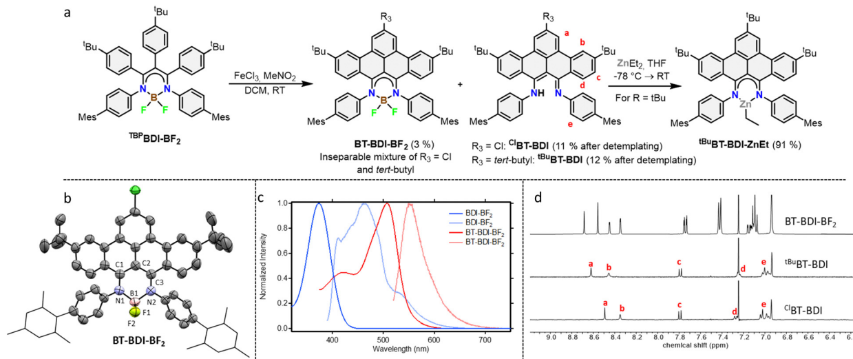
Fig. 2 (a) Reaction scheme showing the reaction of TBP-BDI-BF 2 to form BT-BDI-BF 2 , Cl 1 BT-BDI and t Bu BT-BDI and further reaction of t Bu BT-BDI to form t Bu BT-BDI-ZnEt . (b) Displacement ellipsoid plot (50% probability) of the asymmetric unit of BT-BDI-BF 2 in the crystal. Hydrogen atoms are omitted, and mesityl groups are shown as wireframe for clarity. Only the major disorder component is shown. Severely disordered methyl t -butyl ether molecules are omitted. There is substitutional disorder for the substituents at C47 between chlorine and t -butyl in a ratio of 57.9(4) : 42.1(4). (c) Comparison of the absorption (dark traces) and emission (light traces) spectra of TBP-BDI-BF 2 and BT-BDI-BF 2 measured in DCM (left). For the emission spectra, the sample was excited at the wavelength of the shown absorption maximum. (d) Comparison of the aromatic region of the 1 H NMR spectrum of BT-BDI-BF 2 , t Bu BT-BDI and Cl 1 BT-BDI with relevant assignments corresponding to (a) of this same figure measured in CDCl 3 (right).
